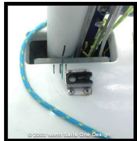
Figure 4 - Mast "neutral" position, note marks in front of and behind neutral mark.
